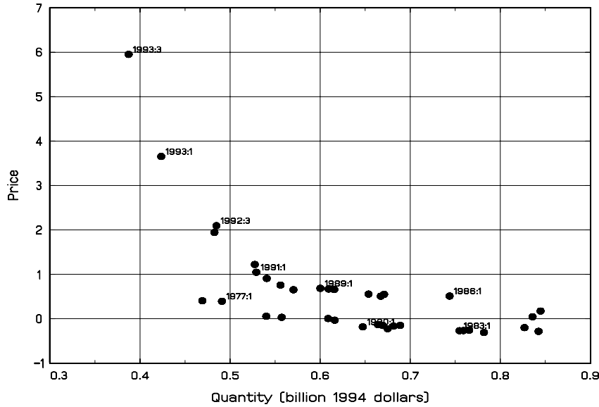
Fig. 3. Industry price-quantity pairs, 1975:1–1993:4.
