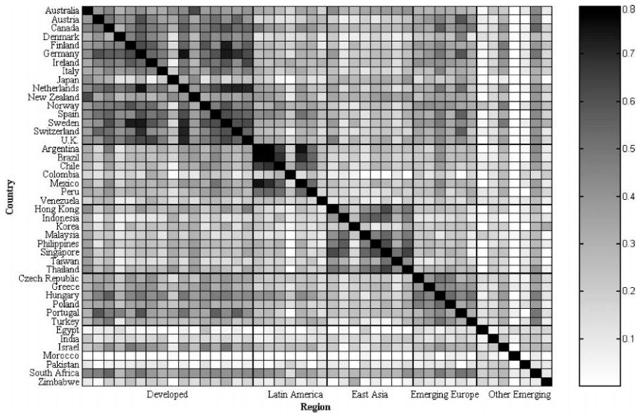
Fig. 4. Heatmap of weekly equity return correlations. The figure summarizes over 900 pairwise correlations. The equity return in U.S. of one country is correlated with the equity return of a second country. The data are from the MSCI local country index, and are multiplied by the exchange rate available from WMR/Reuters from August 1, 1994 to December 31, 1998. Table 5 presents the average pairwise correlation and the associated standard error for each region.
